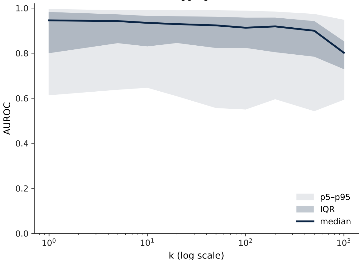
AUROC vs k — aggregated across folds
