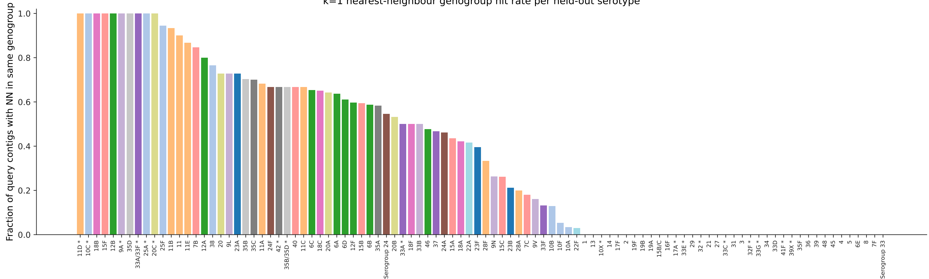
k=1 nearest-neighbour genogroup hit rate per held-out serotype
