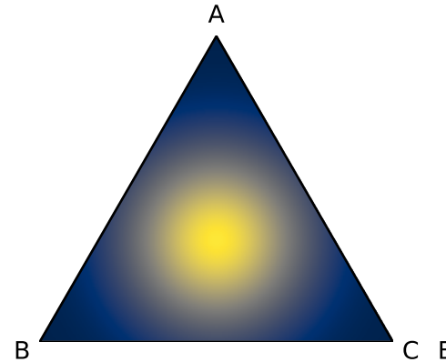
(c) Out-of-distribution
