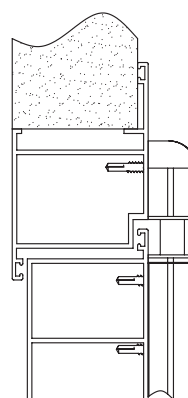
Apertura interna complanare Internal aligned opening
