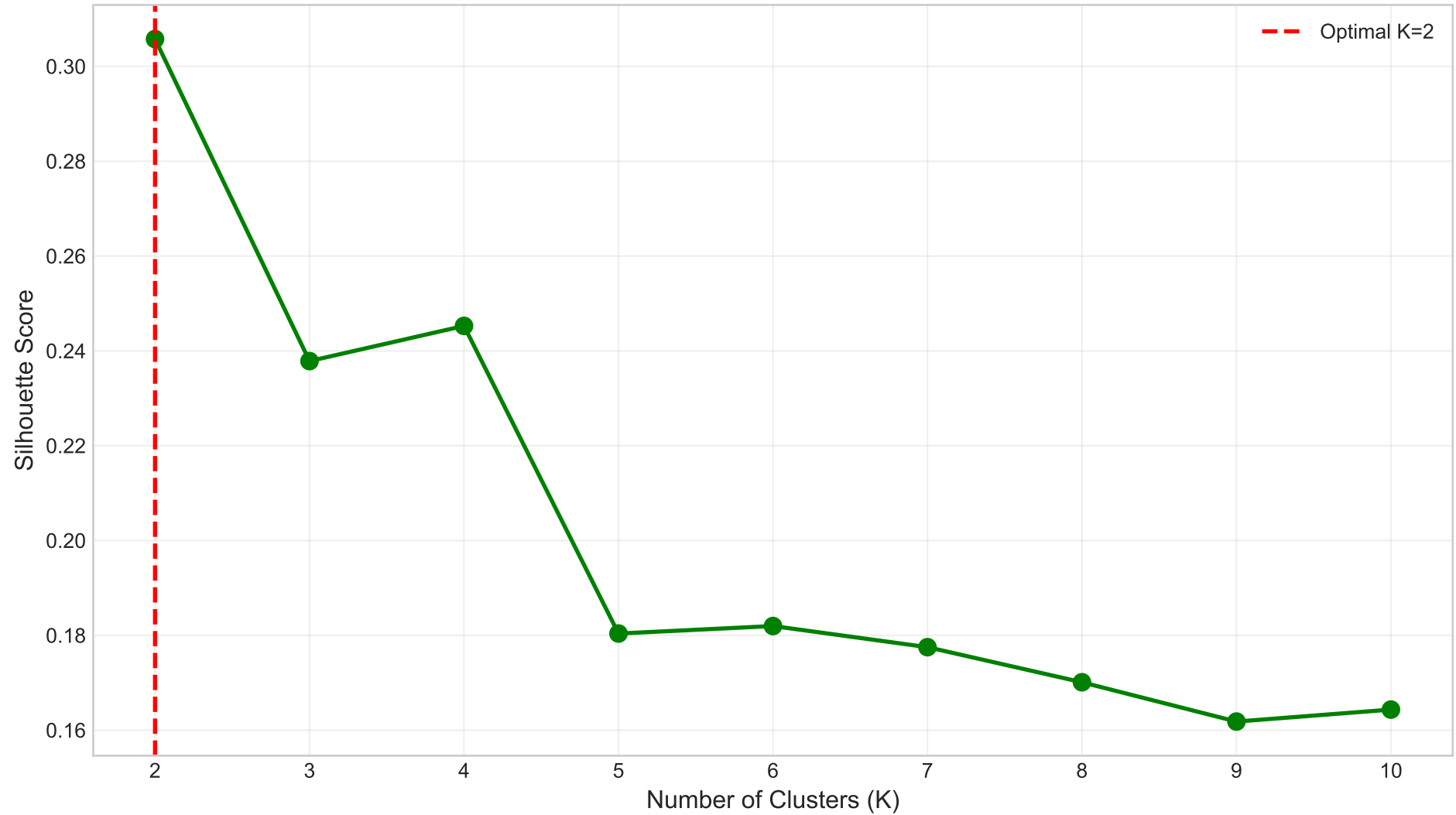
Silhouette Analysis for Optimal K
