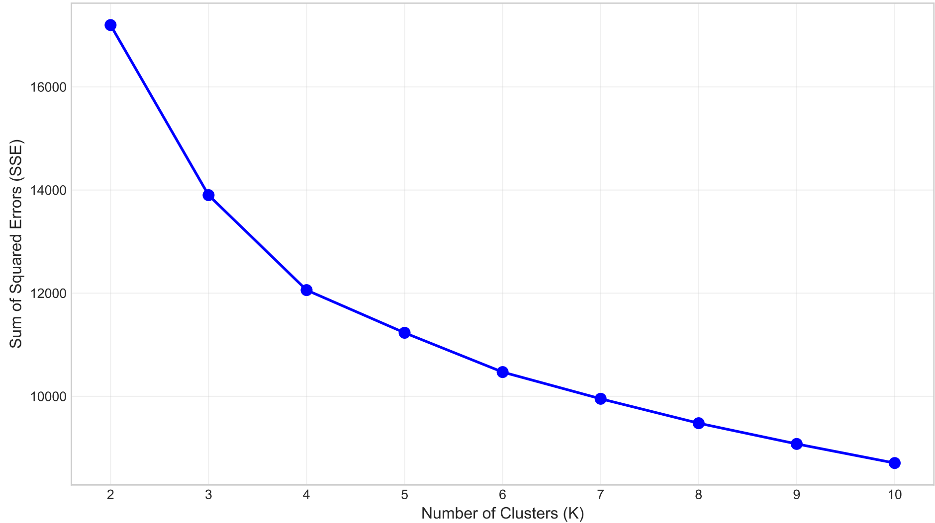
Elbow Method for Optimal K
