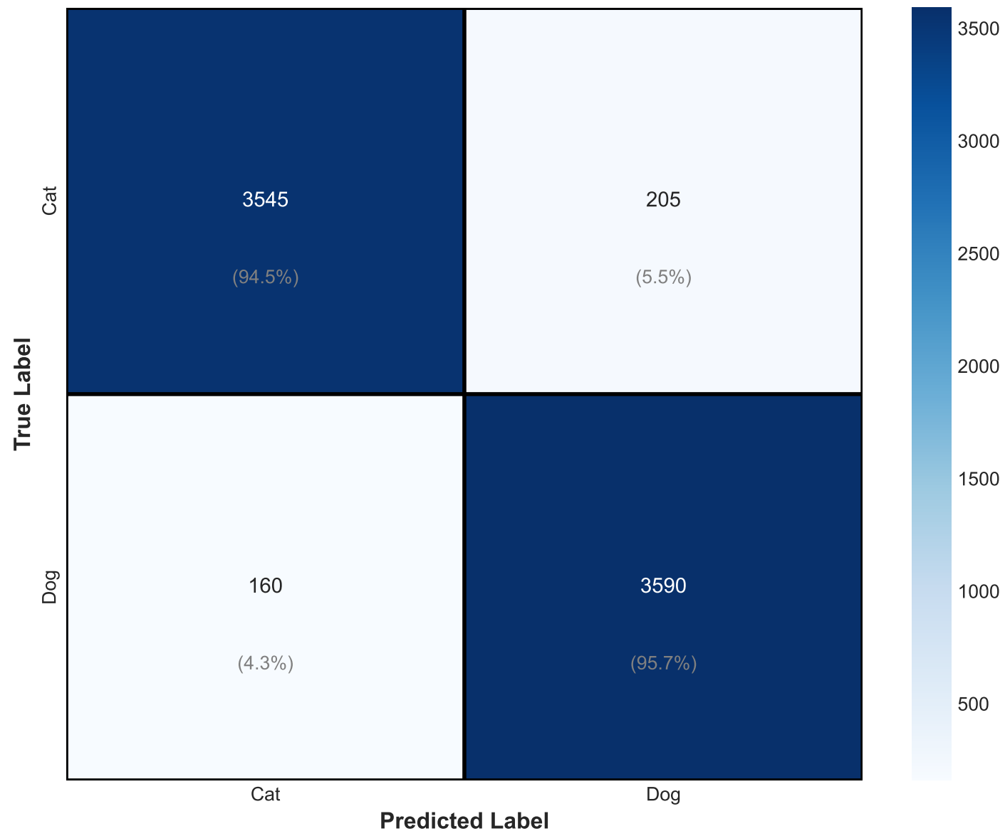
Confusion Matrix (Count and Percentage)
