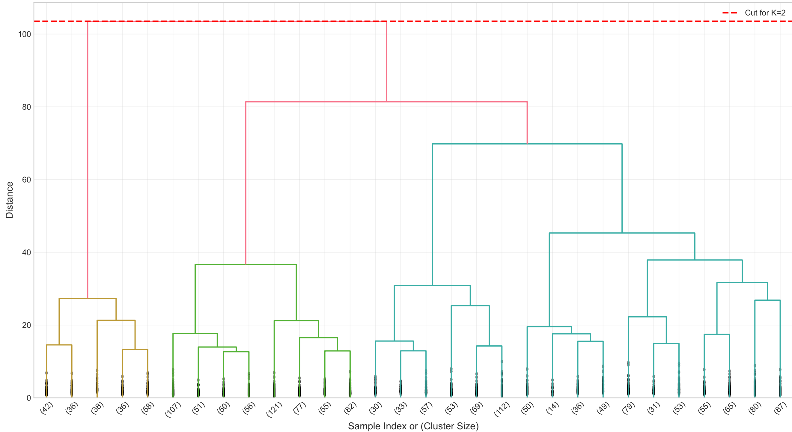
Hierarchical Clustering Dendrogram (ward linkage)
