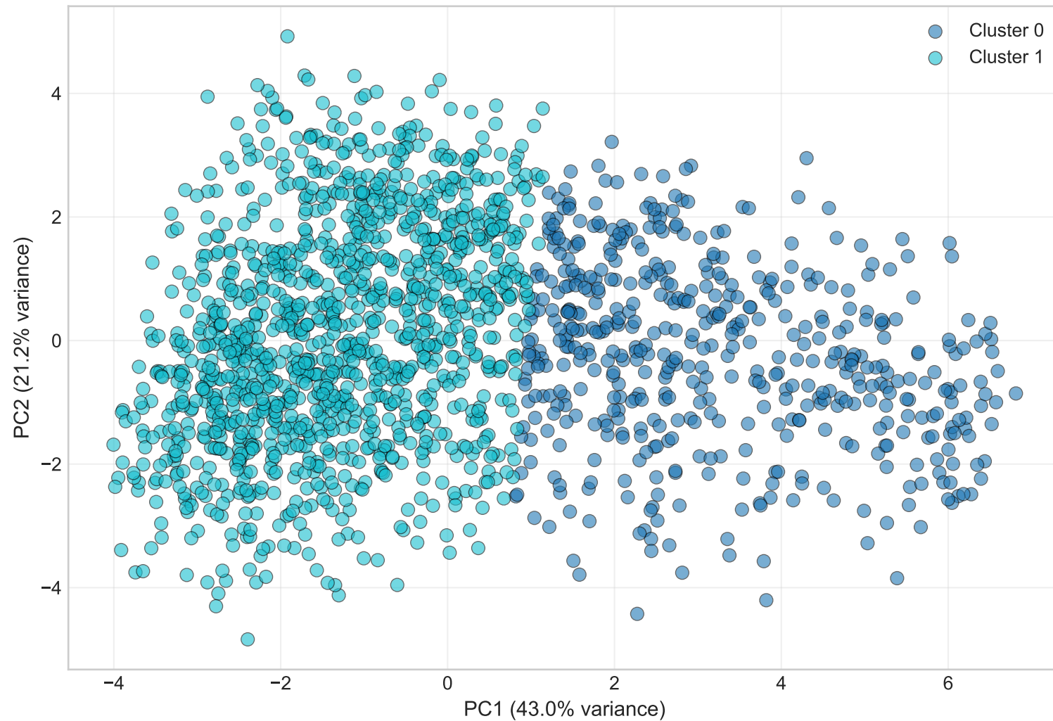
K-Means Clustering (K=2) Silhouette: 0.306
