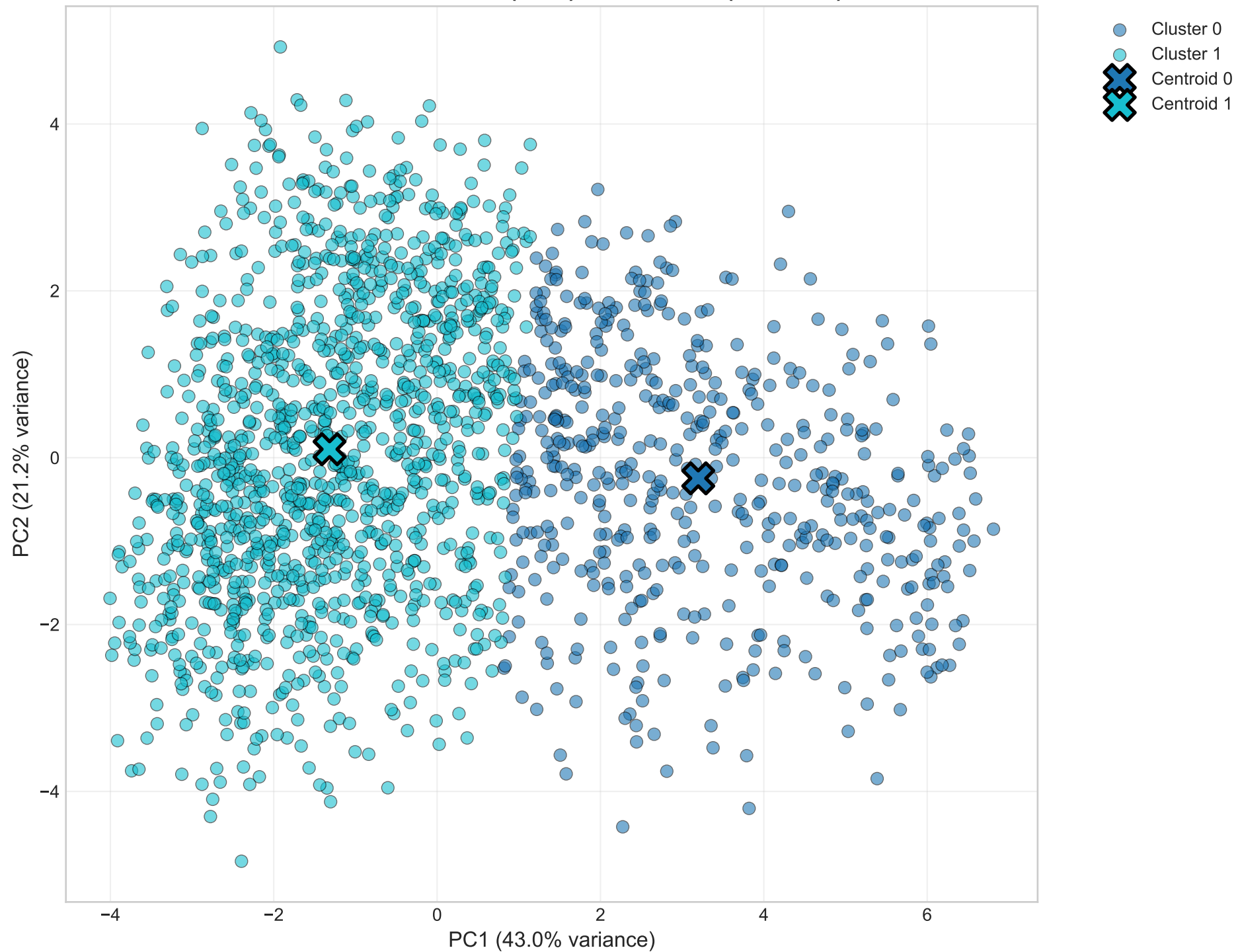
Cluster Visualization (PCA) - 2 Clusters (K-Means)
