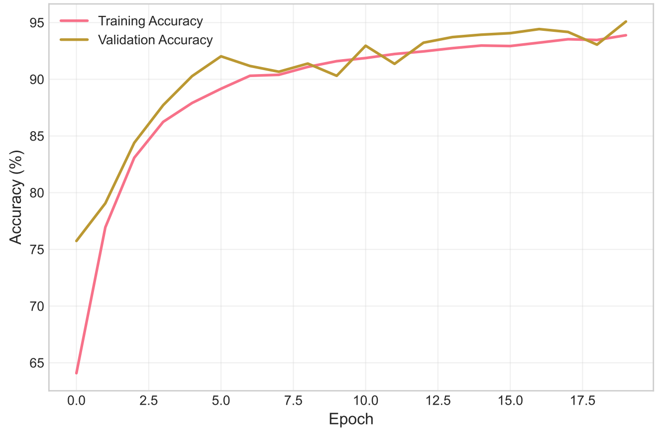
Training and Validation Accuracy
