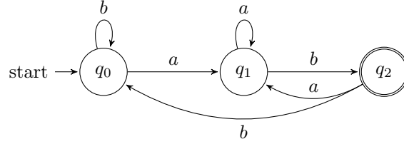
Figure 1: DFA for all words that end with ab .
