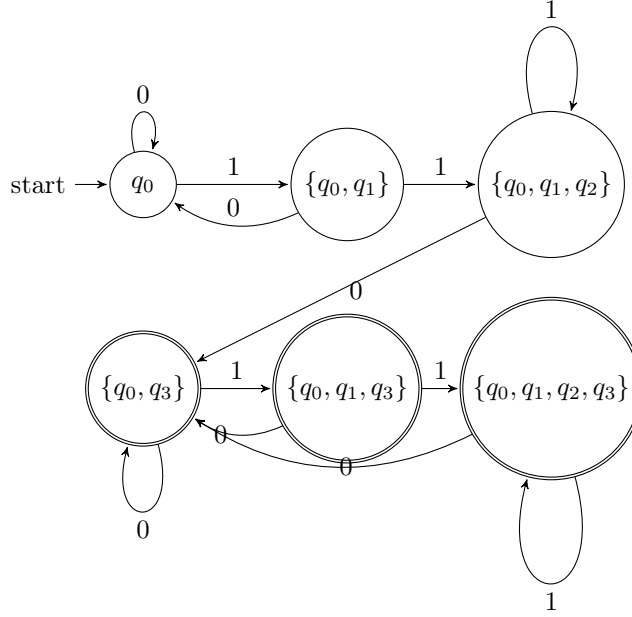
Figure 12: Determinized DFA \mathcal{A}^D for Homework 2 over alphabet \{0,1\} . Accepting states are the subsets that contain the original accepting state q_3 .
