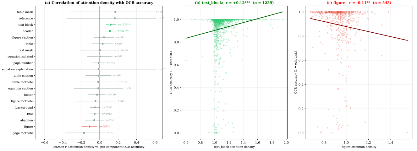
Figure 3. (a) Forest plot of raw Pearson r between per-component attention density and OCR accuracy, with 95% Fisher-z confidence intervals. Green = significant positive ( p < 0.05 ), red = significant negative, grey = n.s. (b–c) Per-document scatter plots for text_block ( r = +0.12 ) and figure ( r = -0.11 ).
