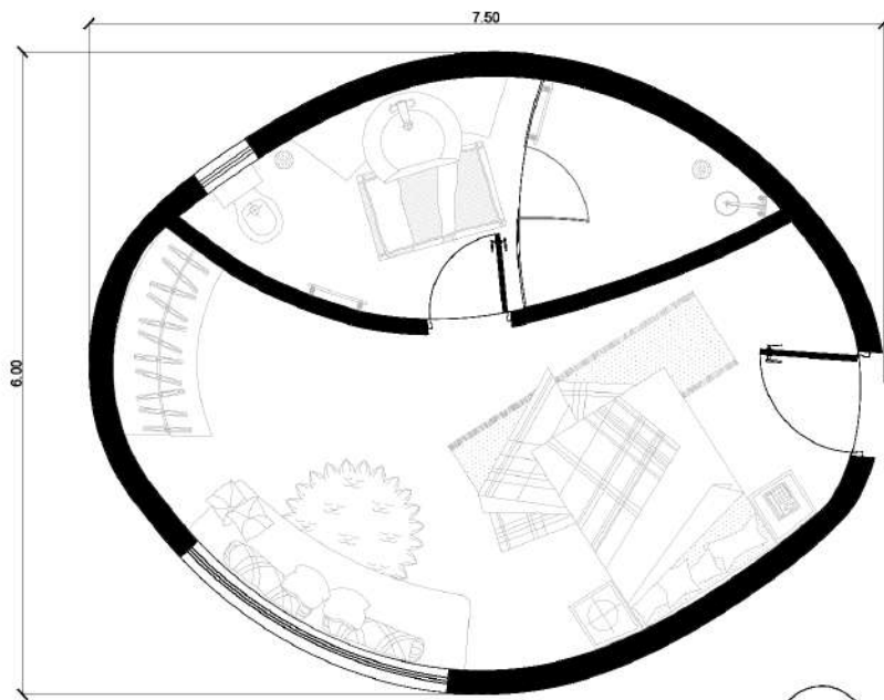
Floor Plan
