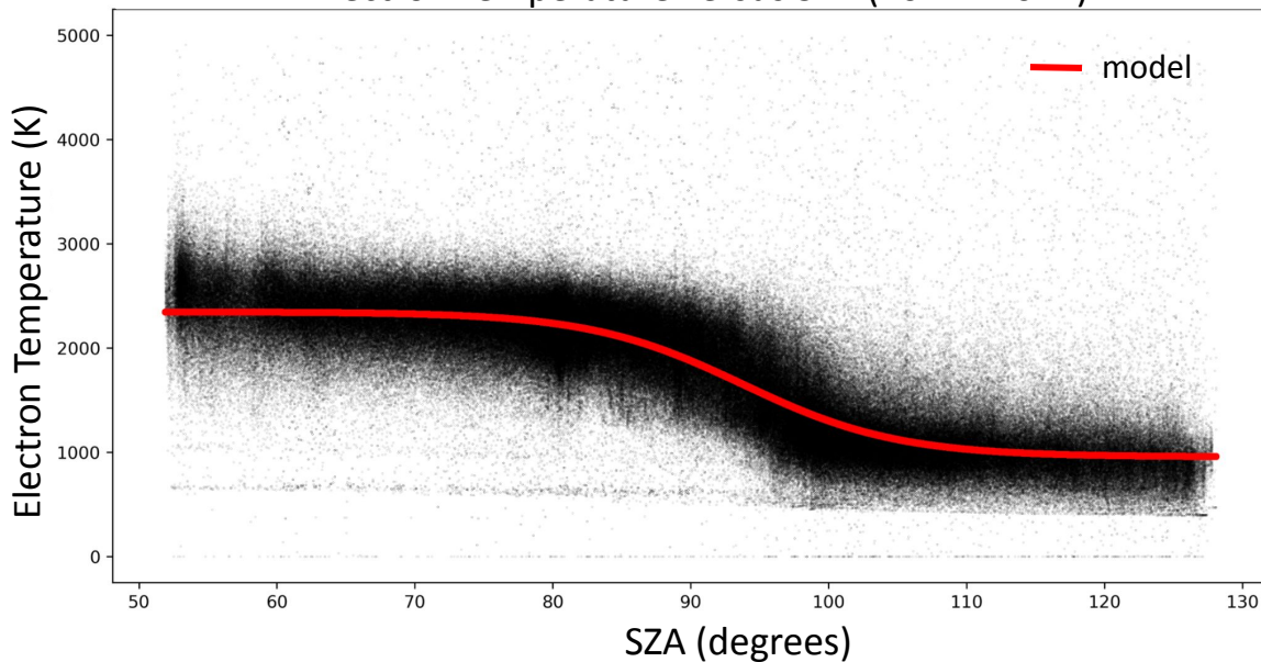
Electron Temperature versus SZA (2012 - 2024)
