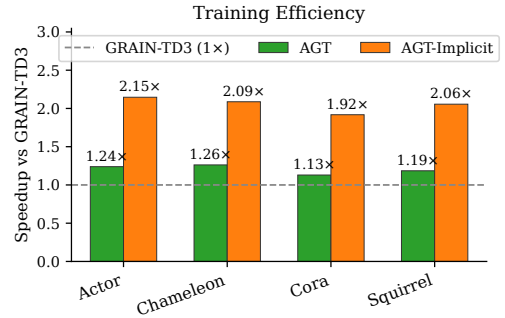
Figure 3: Training speedup of AGT-Implicit compared to GRAIN-TD3.
