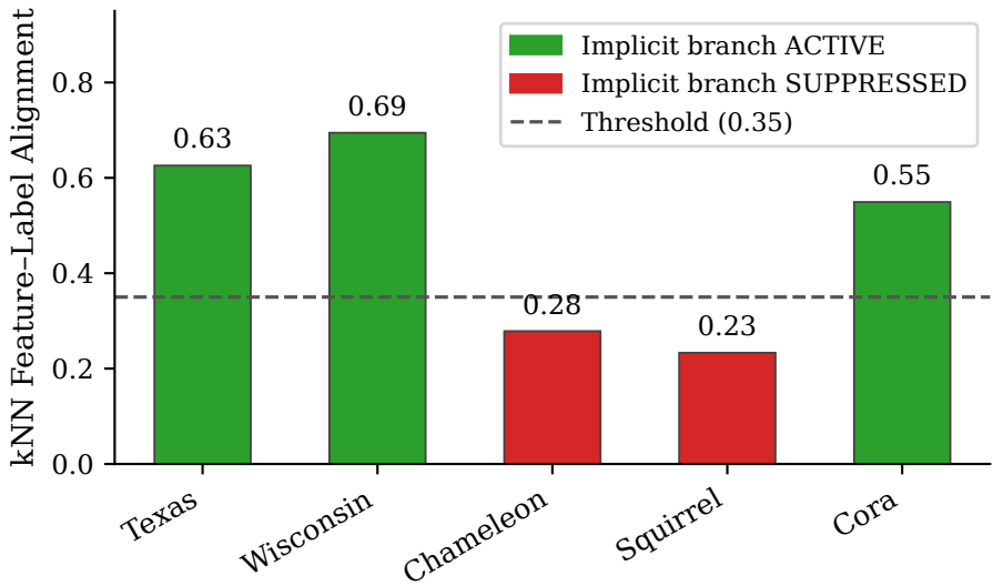
Adaptive Gate: kNN Alignment per Graph
