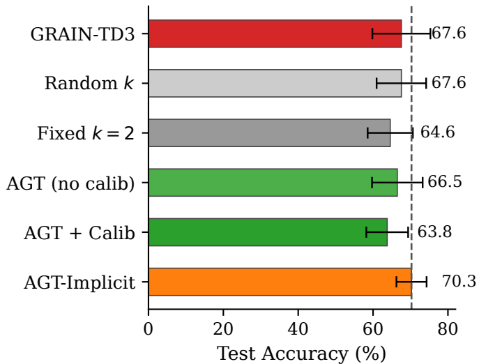
Ablation: Texas
