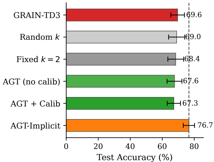
Ablation: Wisconsin
