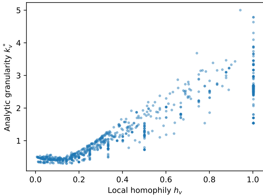
Chameleon — r=0.921
