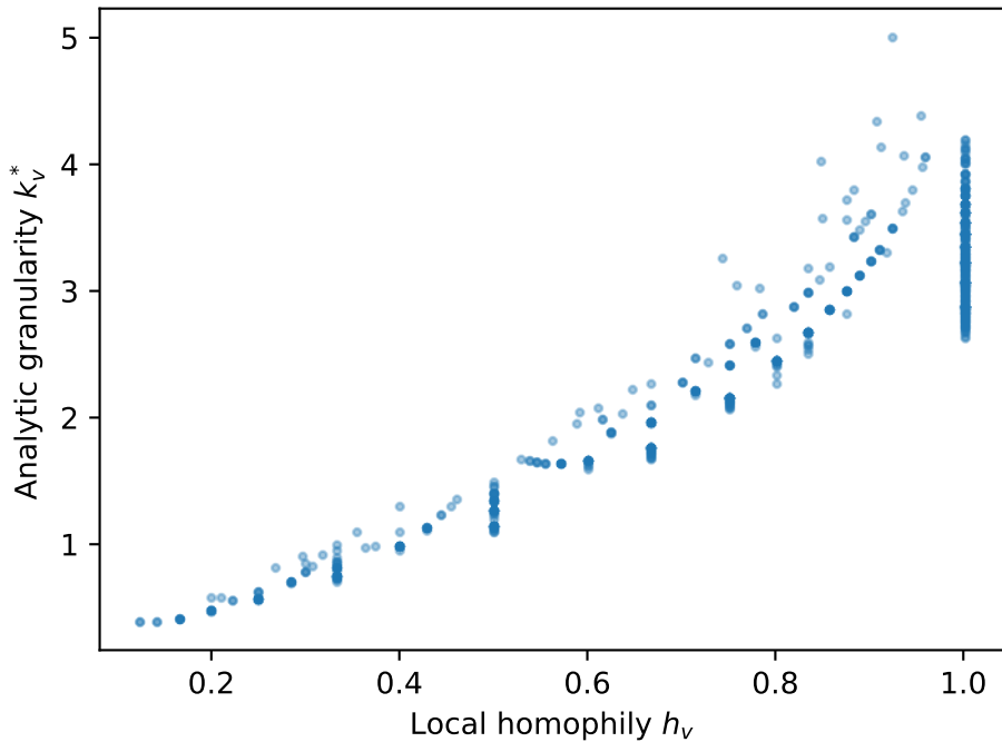
Cora — r=0.951
