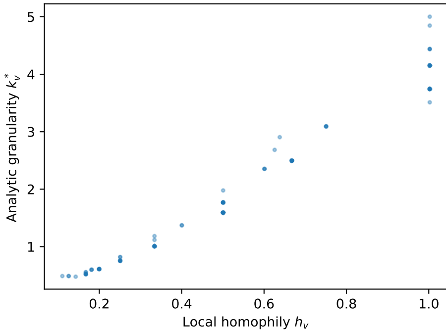
Wisconsin — r=0.988
