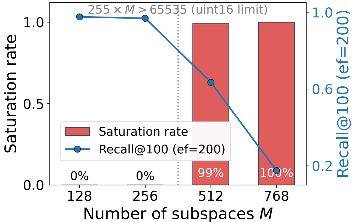
(b) Saturation rate and Recall vs. M (GIST)
