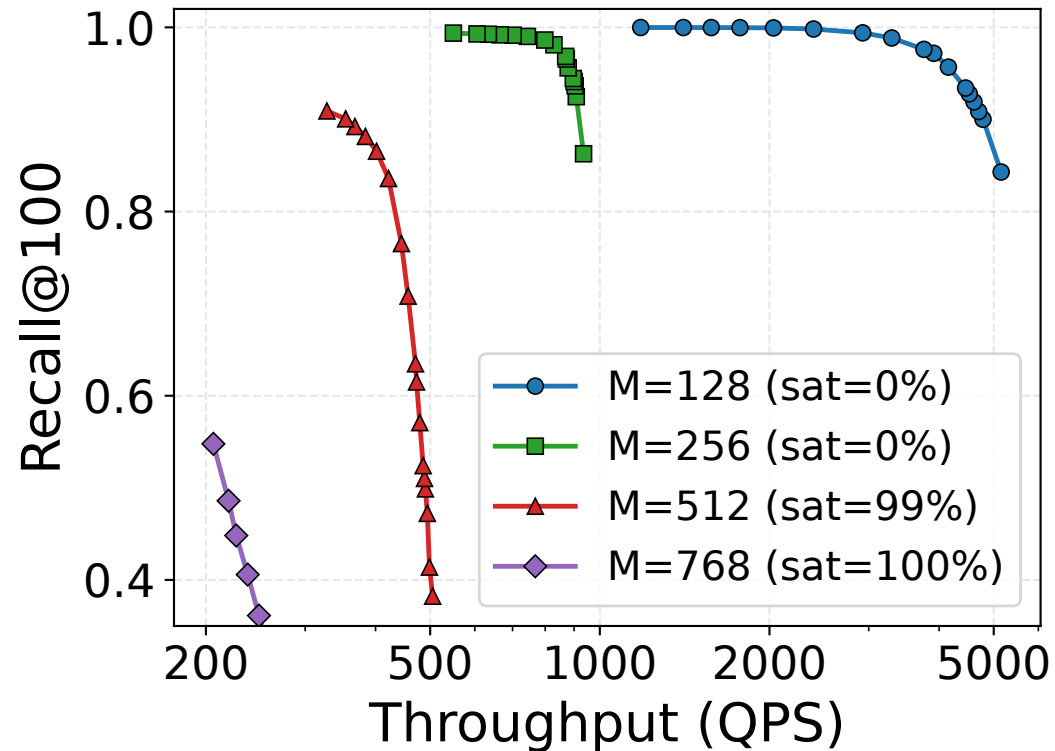
(a) Recall vs. QPS (GIST)
