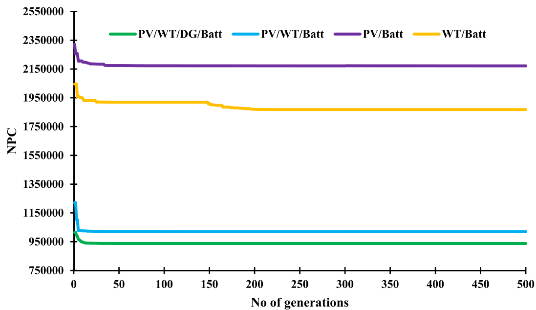
Fig. 5. Convergence of different HES configurations.
