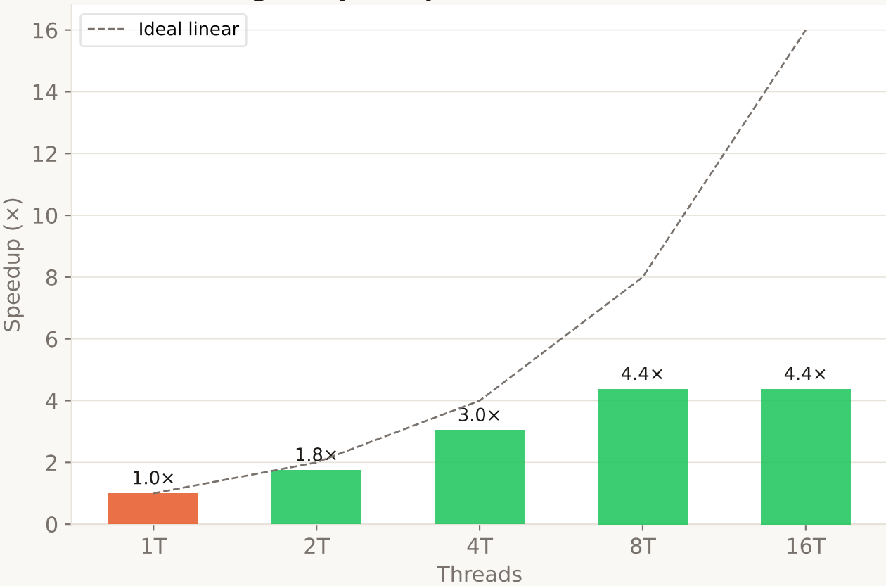
Ingest Speedup vs Serial (46M rows)
