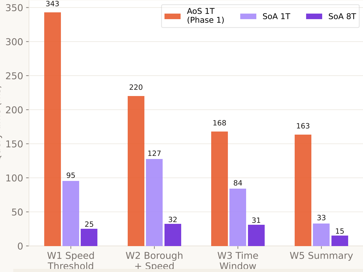
Phase 3 — Query Latency: AoS vs SoA (46M rows)
