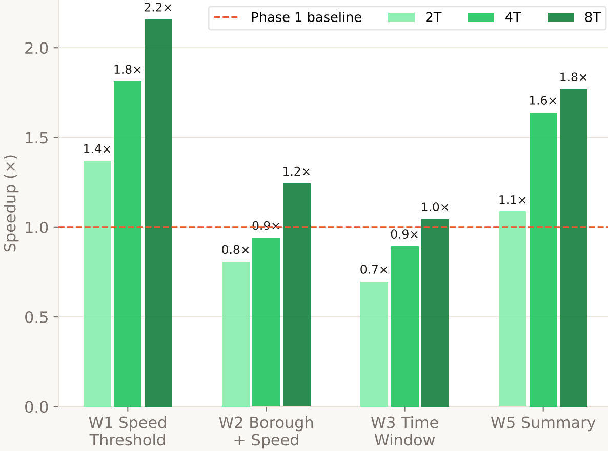
Total Speedup: Phase 3 (SoA + 8T) vs Phase 1 Serial
