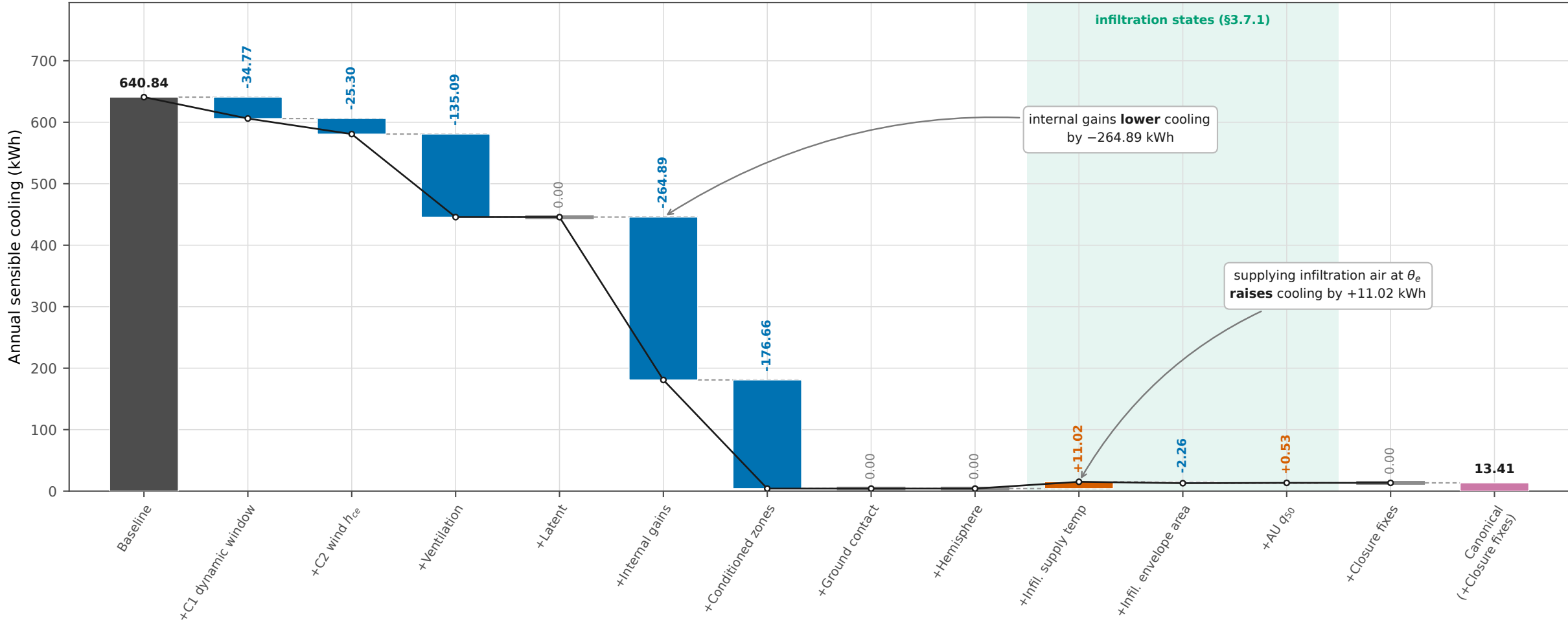
B — Sensible cooling: baseline 640.84 kWh → canonical 13.41 kWh
