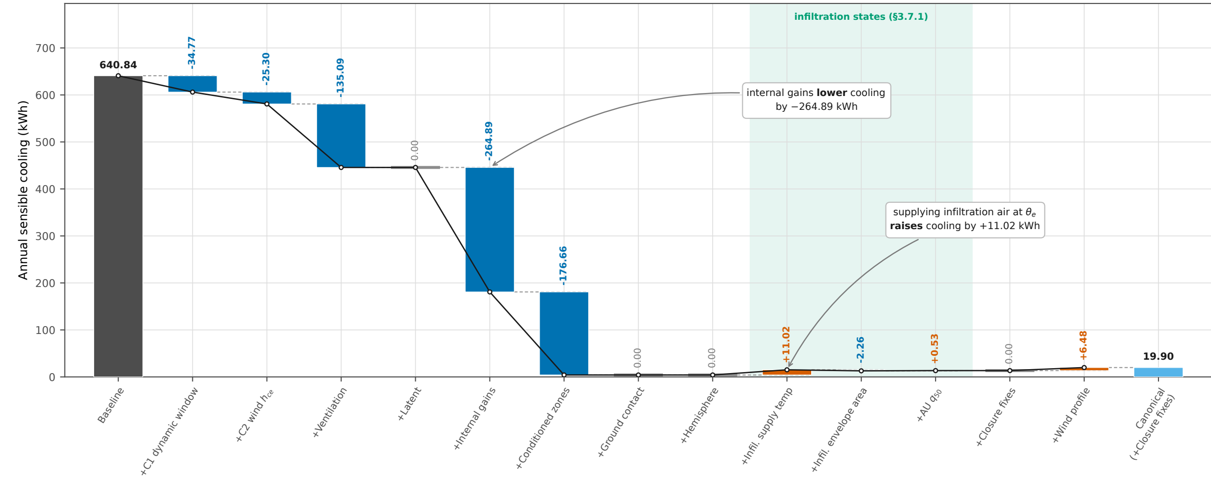
B — Sensible cooling: baseline 640.84 kWh → canonical 19.90 kWh
