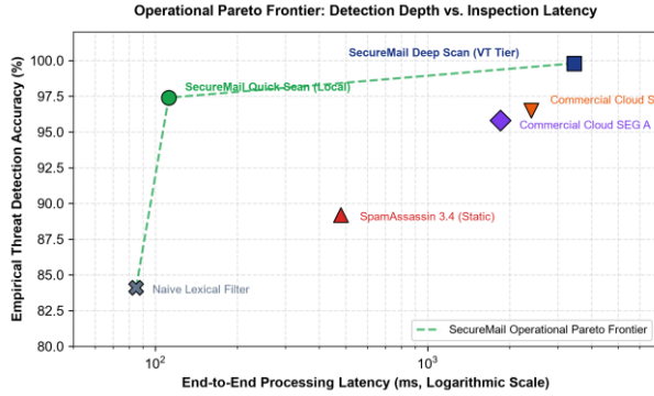
Fig. 19. Operational Pareto Frontier Quantifying Empirical Detection Depth versus End-to-End Processing Latency.
