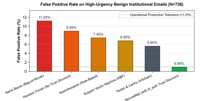
Fig. 11. False Positive Rate on High-Urgency Benign Institutional Emails (N=738) Contrasting Classical Classifiers against SecureMail Provenance Discount.
