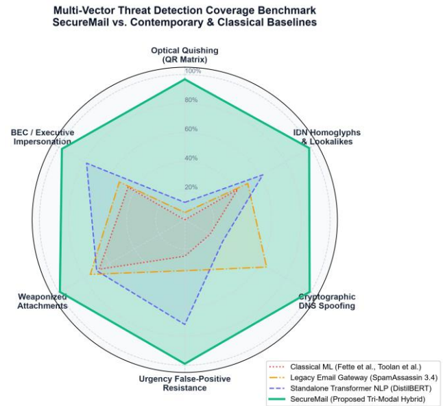
Fig. 16. Multi-Vector Threat Detection Coverage Benchmark Contrasting SecureMail against Contemporary and Classical Baselines across Six Attack Vectors.
