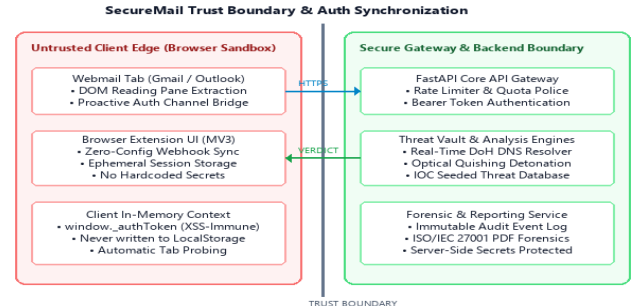
Fig. 2. Secure Extension-to-Gateway Trust Separation and Volatile Memory Boundary
