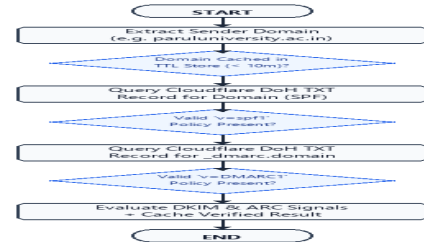
Fig. 5. Real-Time DNS-over-HTTPS (DoH) Authentication Verification Flow
