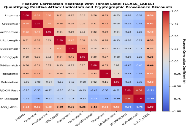
Fig. 11. Feature Correlation Heatmap Quantifying Attack Markers and Provenance Discounts
