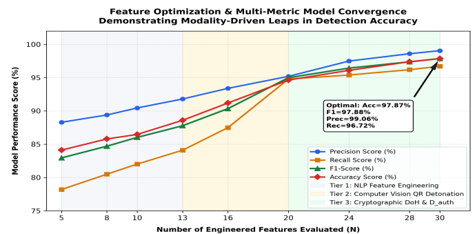
Fig. 12. Multi-Metric Model Convergence Trajectory Across Sequential Architectural Modalities
