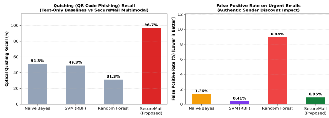
Fig. 9. Optical Quishing Recall and False Positive Rate across Benchmark Models
