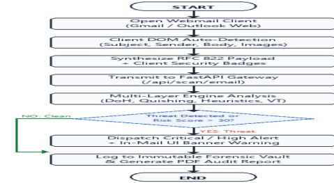
Fig. 4. End-to-End Threat Detection and Forensic Ingestion Flow
