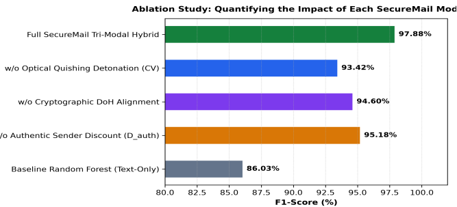
Fig. 10. Ablation Study Quantifying the Impact of Individual SecureMail Modalities
