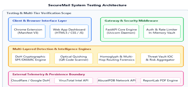
Fig. 1. SecureMail System Testing Architecture and Multi-Layer Operational Boundaries
