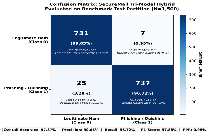
Fig. 13. Confusion Matrix on Benchmark Test Partition (N=1,500)
