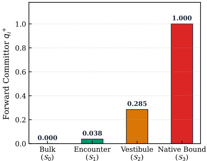
(a) TPT Committor Distribution
