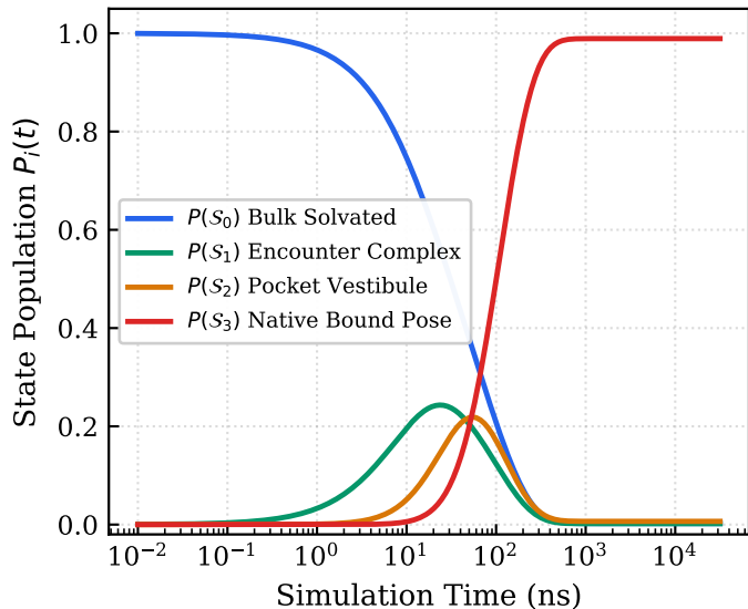
(b) Master Equation Kinetic Relaxation
