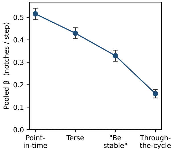
(b) Instruction gradient (pooled)
