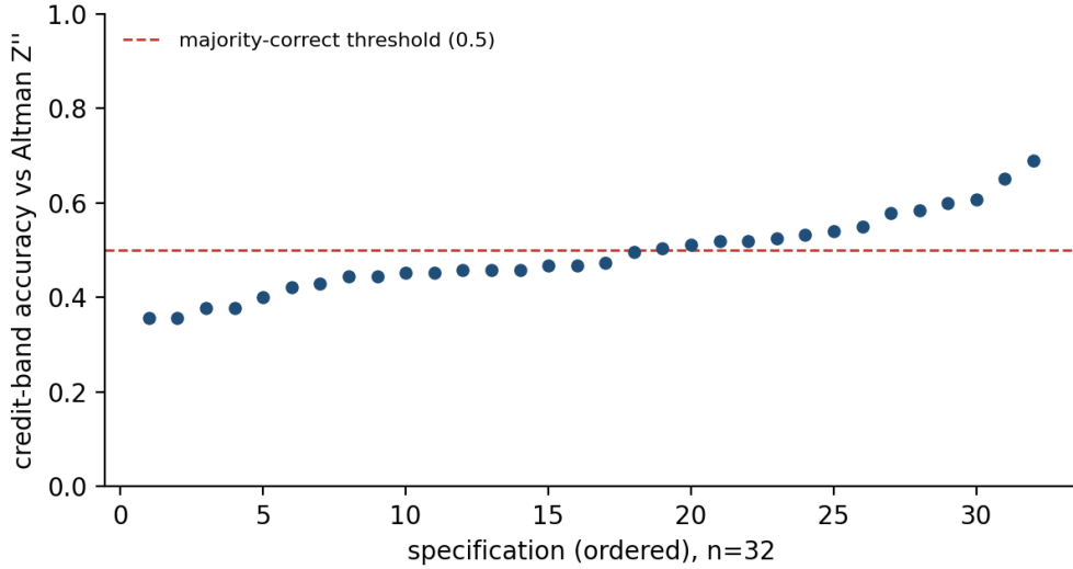
Figure 1: Specification curve of the machine credit rating. Each point is one of the pre-registered specifications (three seeds pooled), ordered by majority-correct credit-band accuracy against the Altman Z'' benchmark. Accuracy ranges widely across specifications despite identical firm fundamentals, and roughly half reverse the pre-registered accuracy verdict—the multiverse the method is named for.
