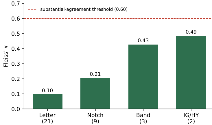
Figure 3: Chance-corrected cross-specification agreement (Fleiss \kappa ) by granularity; agreement never reaches the \kappa = 0.6 substantial-agreement threshold, peaking at 0.49 on the IG/HY split.
