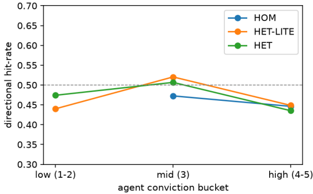
FIGURE 5. Self-reported conviction does not predict directional accuracy. Per-agent directional hit-rate by self-reported conviction bucket; no configuration rises reliably above chance (0.5, dashed), consistent with the secondary directional-accuracy analysis.
