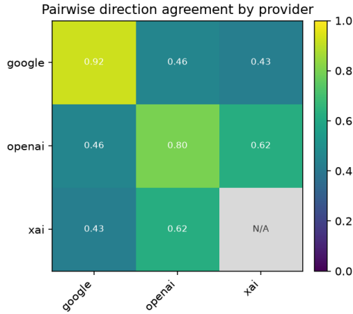
FIGURE 4. Pairwise directional-agreement matrix by provider. Diagonal (within-provider) agreement greatly exceeds off-diagonal (cross-provider), which is where the reduction in ensemble agreement originates. The xAI–xAI diagonal is undefined (marked N/A, not 0): each HET cell contains a single xAI agent, so no within-xAI agent pair exists.
