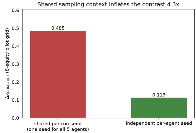
FIGURE 3. Effect of seeding protocol on the pilot HOM – HET agreement contrast. The contrast is 0.485 under a shared seed and 0.113 under distinct per-agent seeds. Both estimates use the same pilot grid and model set.
