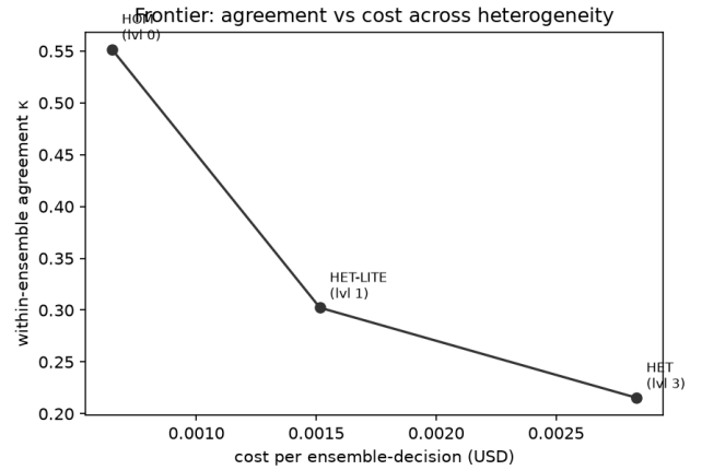
FIGURE 1. Agreement–cost frontier. Within-ensemble Fleiss' \kappa ( y ) versus cost per ensemble decision ( x ) at heterogeneity levels \{0, 1, 3\} . Lower \kappa indicates lower observed within-ensemble agreement; the horizontal spread is the cost premium.
