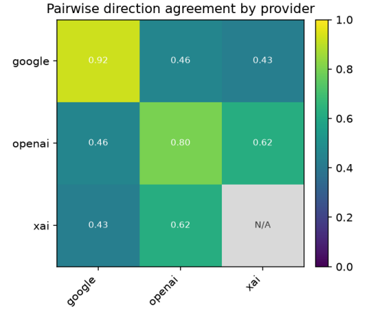
FIGURE 4. Pairwise directional-agreement matrix by provider. Diagonal (within-provider) agreement greatly exceeds off-diagonal (cross-provider), which is where the reduction in ensemble agreement originates. The xAI–xAI diagonal is undefined (marked N/A, not 0): each HET cell contains a single xAI agent, so no within-xAI agent pair exists.
