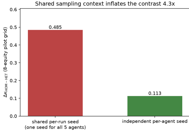
FIGURE 3. Effect of seeding protocol on the pilot HOM–HET agreement contrast. The contrast is 0.485 under a shared seed and 0.113 under distinct per-agent seeds. Both estimates use the same pilot grid and model set.
