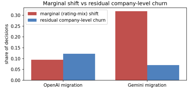
FIGURE 2. Prevalence decomposition of the gross flip into a marginal (rating-mix) shift and residual company-level churn. OpenAI is churn-dominated; Gemini is marginal-dominated.
