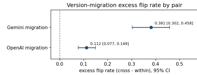
FIGURE 1. Excess flip rate (cross-version minus within-version noise floor) with 95% CI for both migrations; both intervals exclude zero.
