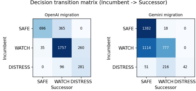
Figure 3: Decision transition matrices ( v_{\text{old}} \rightarrow v_{\text{new}} ) for each migration. OpenAI’s mass moves off the diagonal toward more-severe tiers; Gemini’s moves sharply into SAFE.
