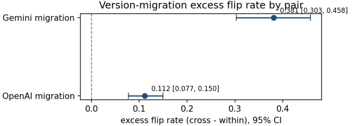
Figure 1: Excess flip rate (cross-version minus within-version noise floor) with 95% CI for both migrations; both intervals exclude zero.
