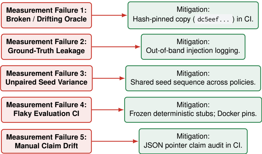
Figure 13: Measurement System Threat Model and Architectural Mitigations.
