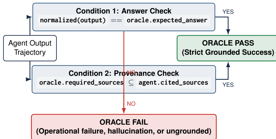
Figure 4: The Dual-Gate Programmatic Oracle. Success requires simultaneous satisfaction of exact token correctness AND complete source provenance.
