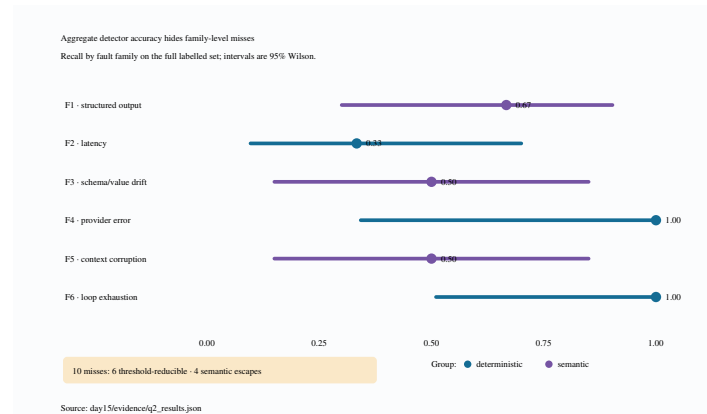
Figure 8: Detector Recall and Confidence Intervals by Fault Family. While aggregate precision was 1.0, micro recall was 0.615, concealing 10 false negatives (4 semantic escapes).
