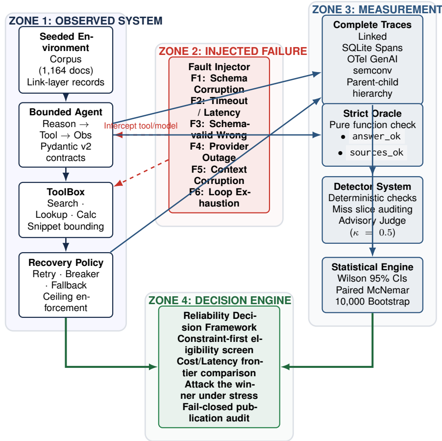
Figure 3: FAULTLINE System Architecture. The experimental workbench enforces strict physical and logical boundaries: the Injected Failure system creates reproducible degradation, the Observed System executes bounded recovery policies, the Measurement System scores outcomes without relying on LLM self-evaluation, and the Decision Engine filters policies through constraint-first Pareto frontiers.
