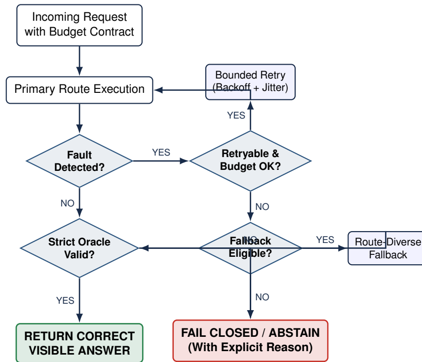
Figure 6: The Enforced Recovery Control Path. Budget ceilings and correctness gates take strict priority over raw availability.
