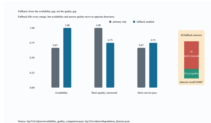
Figure 10: Availability vs Strict Quality Under Primary Provider Outage. Fallback restores availability from 0.667 to 1.0, but strict answer quality drops from 1.0 to 0.75 (30 of 40 fallback answers degraded).
