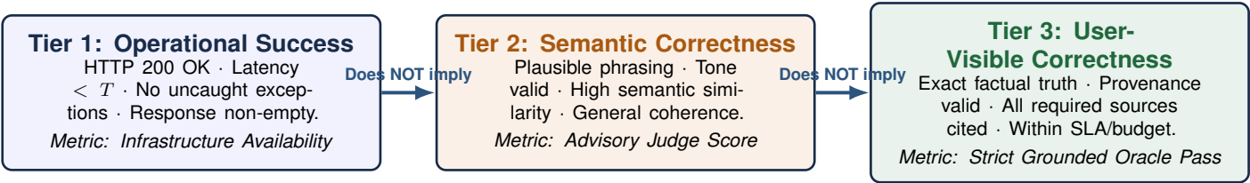
Figure 2: The Three Tiers of Reliability. Conventional systems measure Tier 1 and assume Tier 3. FAULTLINE measures all three independently and forbids promoting Tier 1 or Tier 2 to Tier 3.
