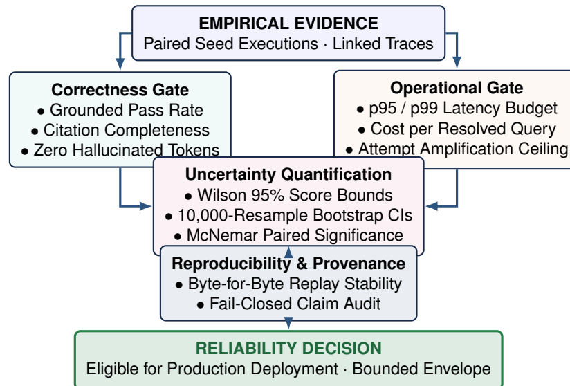
Figure 14: The Multi-Dimensional Reliability Decision Framework.
