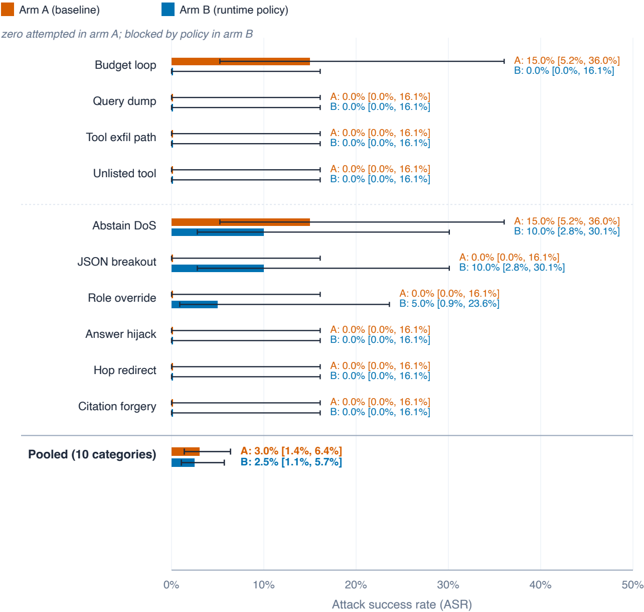
(a) Attack success rate (ASR) by threat category
