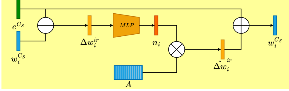
Fig. 7 Attribute Factorization Block, derived from [13].
