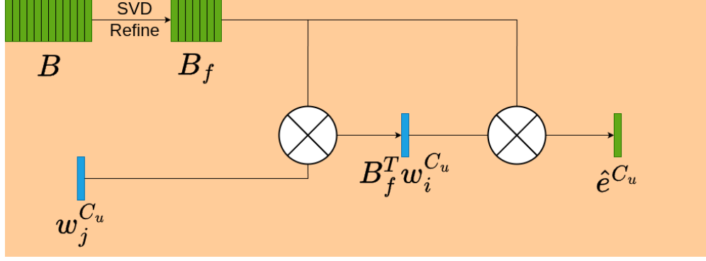
Fig. 8 Class Embedding Block, adapted from [13].
