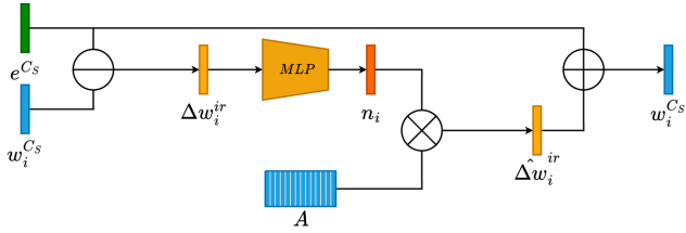
Fig. 7. Attribute Factorization Block, derived from [11]
