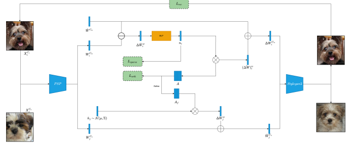
Fig. 2. Attribute Group Editing Framework
