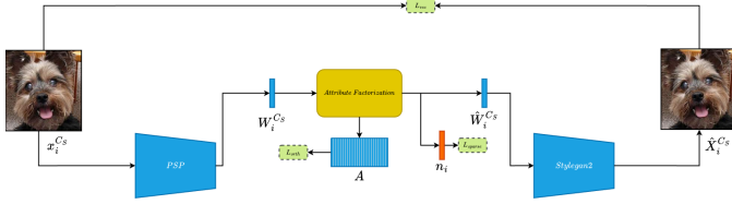
Fig. 6. Attribute Factorization Training Framework [11]
