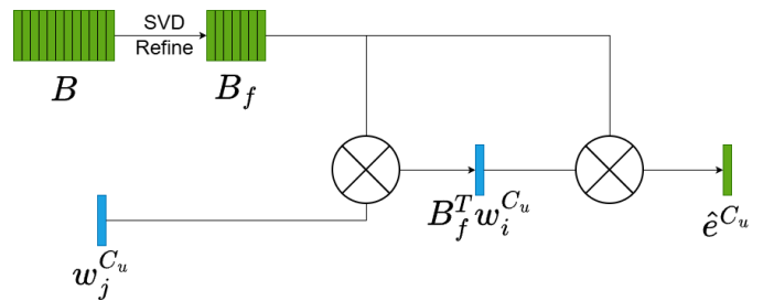
Fig. 8. Class Embedding Block, adapted from [11]
