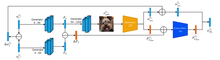
Fig. 10. Feature Editing Decoder Block
