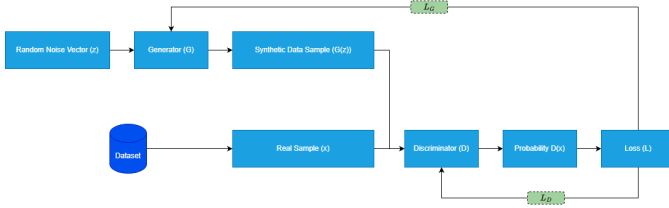
Fig. 1. Generative Adversarial Networks (GANs) Architecture
