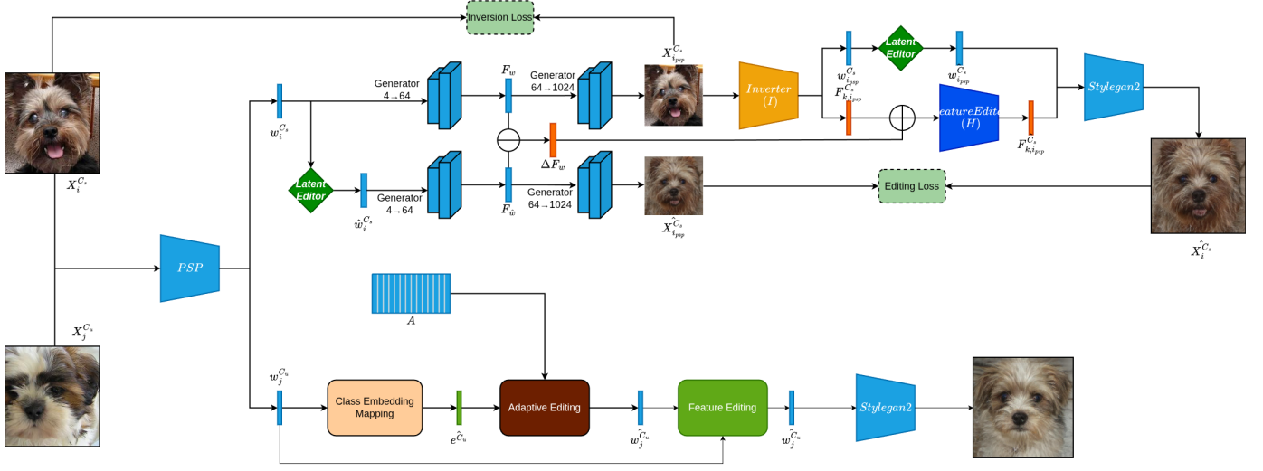
Fig. 5. FeatureSAGE framework
