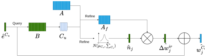
Fig. 9. Adaptive Editing Block, from [11]
