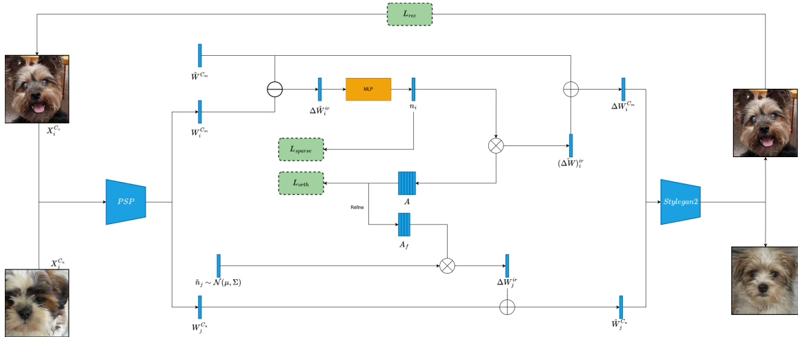
Figure 2-2. Attribute Group Editing framework
