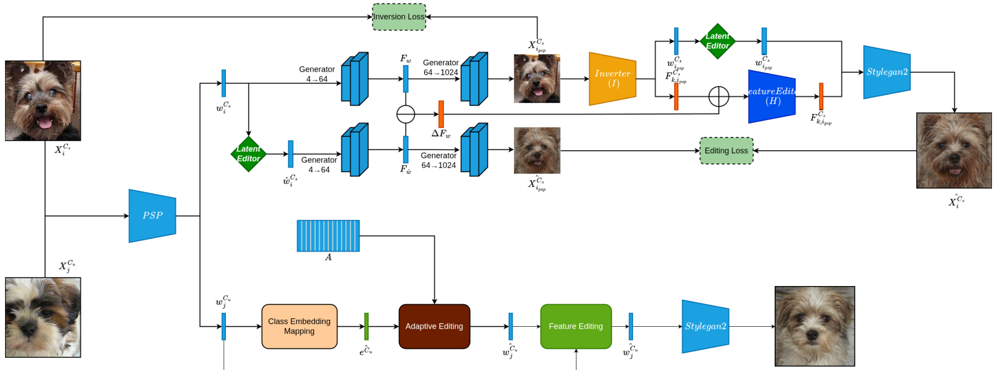
Figure 3.5 FeatureSAGE framework
