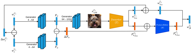
Fig. 10. Feature Editing Decoder Block
