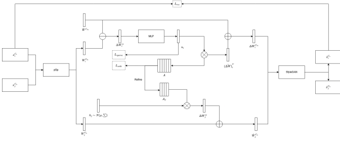
Fig. 2. Attribute Group Editing Framework
