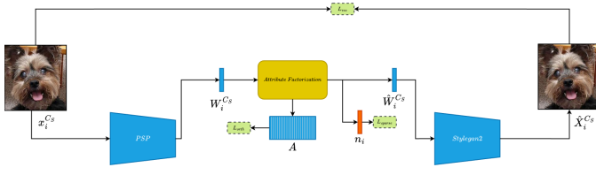
Fig. 6. Attribute Factorization Training Framework [11]
