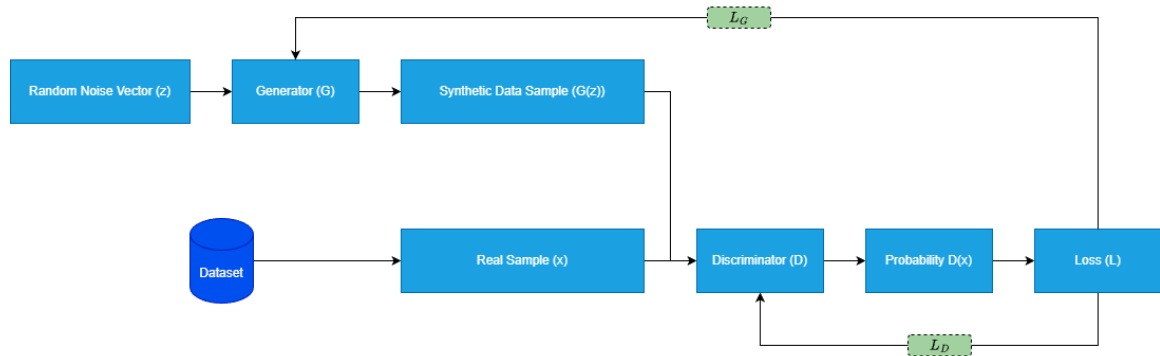
Figure 2-1. Generative Adversarial Networks (GANs) architecture
