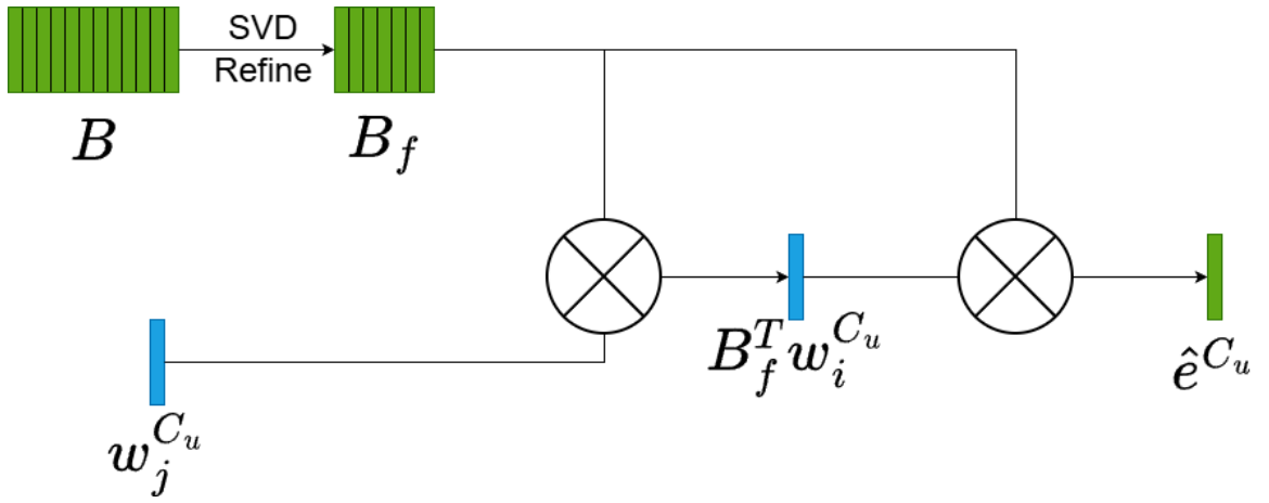
Figure 3-6. Class Embedding Block, adapted from (Ding et al., 2023)
