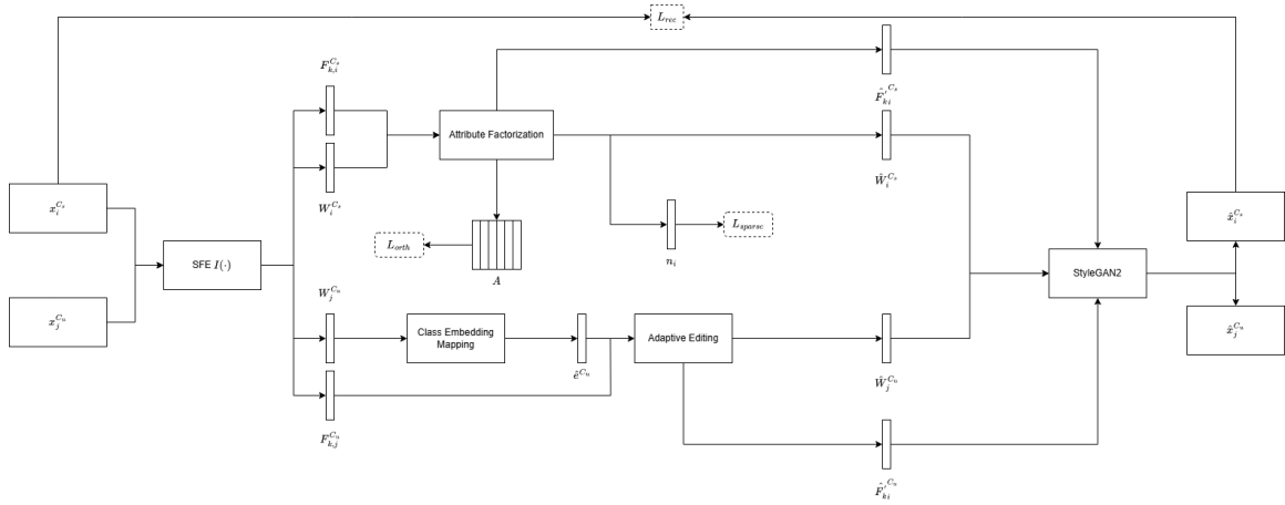
Figure 3.5 FeatureSAGE framework
