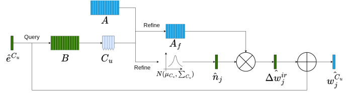
Fig. 9. Adaptive Editing Block, from [11]
