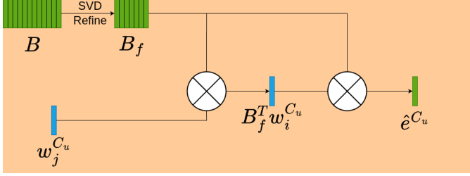
Fig. 8. Class Embedding Block, Adapted from [11]
