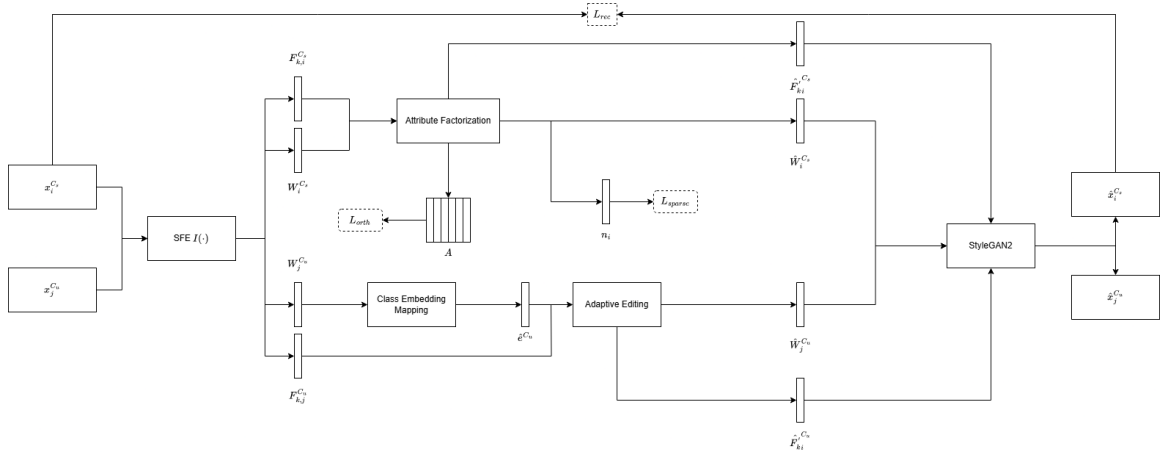
Figure 3.5 FeatureSAGE framework
