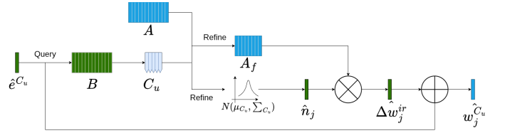
Fig. 9. Adaptive Editing Block, from [?]
