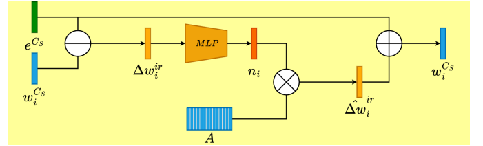
Fig. 7. Attribute Factorization Block, Derived from [?]
