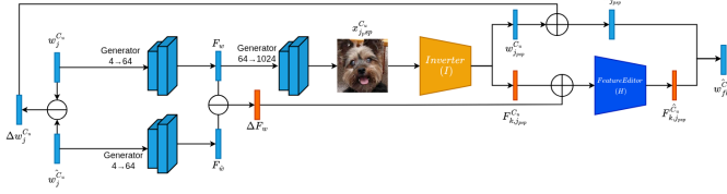
Fig. 10. Feature Editing Decoder Block
