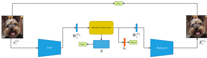
Fig. 6. Attribute Factorization Training Framework [?]
