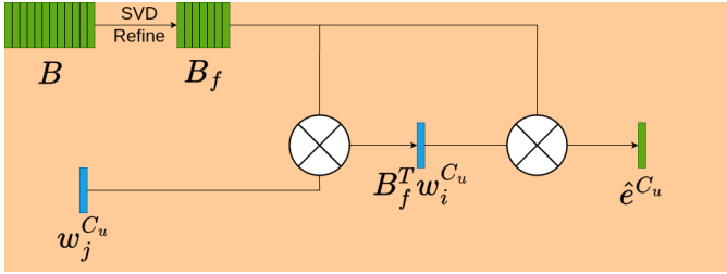
Fig. 8. Class Embedding Block, Adapted from [?]
