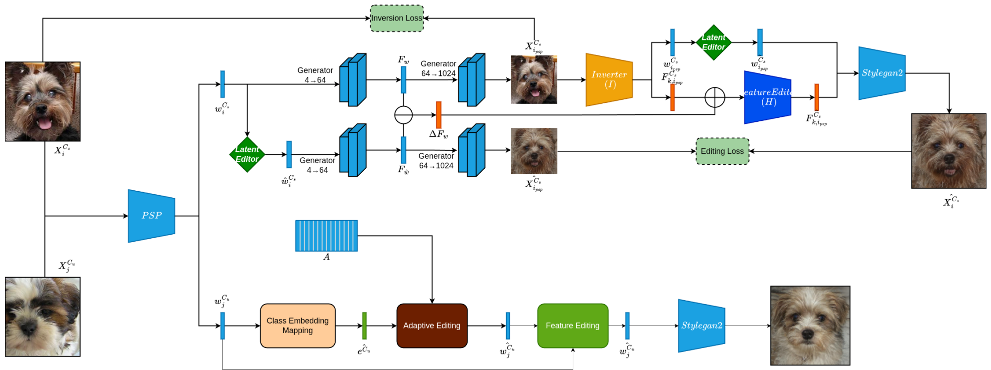
Figure 3.3 FeatureSAGE framework
