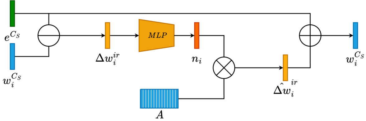
Figure 3-5. Attribute Factorization Block, derived from (Ding et al., 2023)
