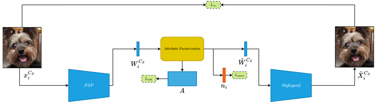
Figure 3-4. Attribute Factorization Training Framework (Ding et al., 2023)
