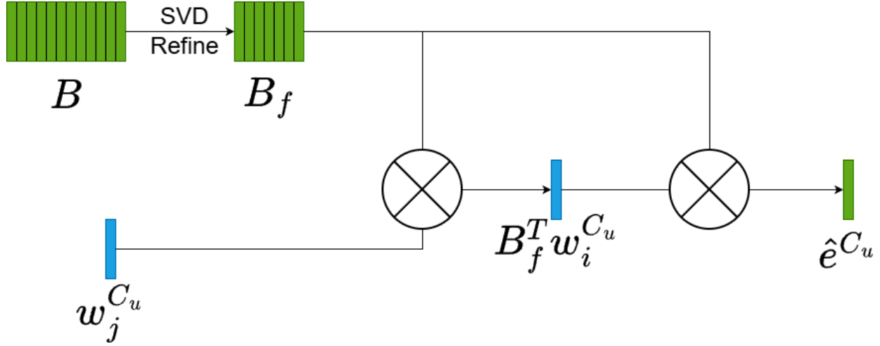
Figure 3-6. Class Embedding Block, adapted from (Ding et al., 2023)
