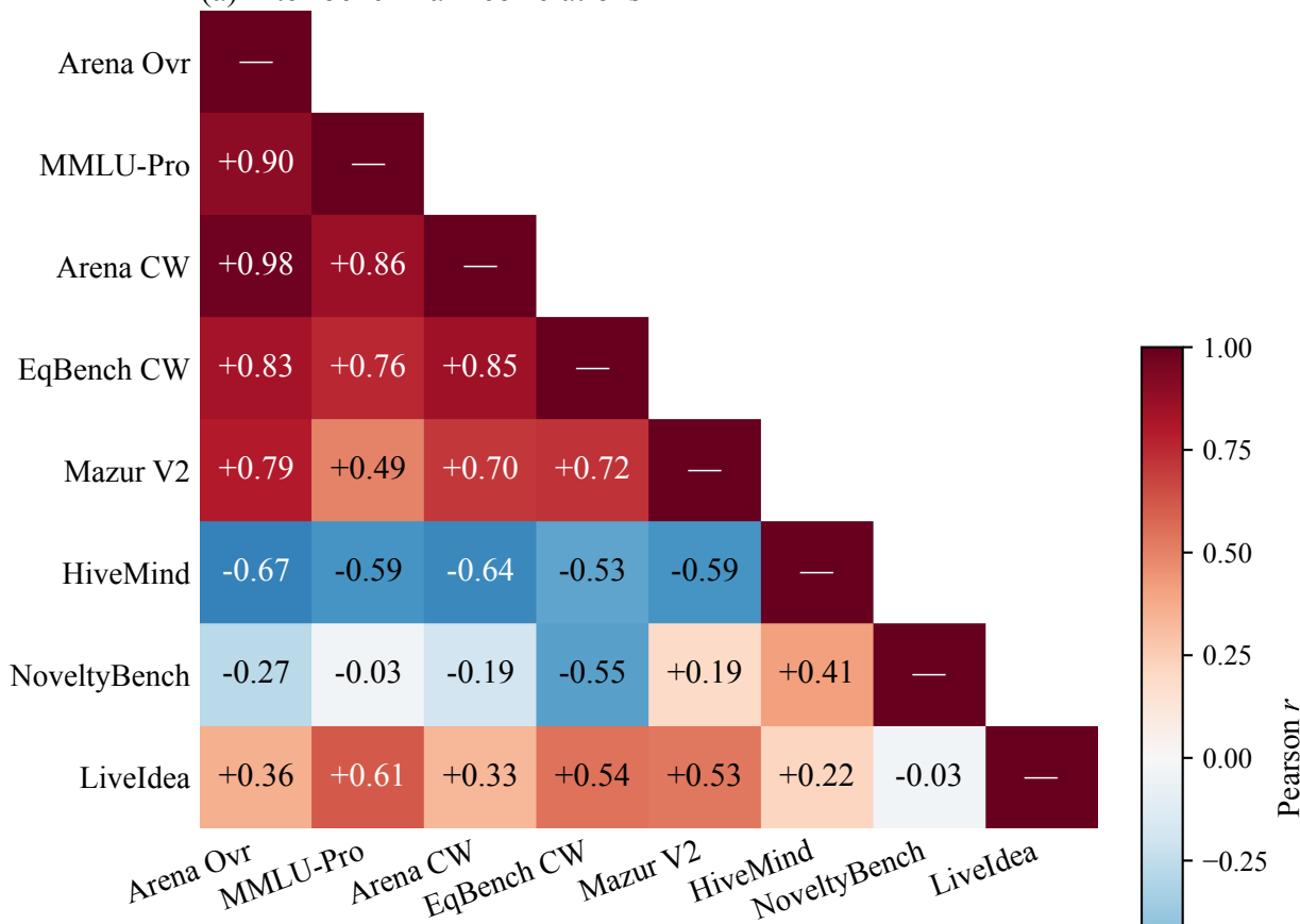
(b) Inter-test correlations
