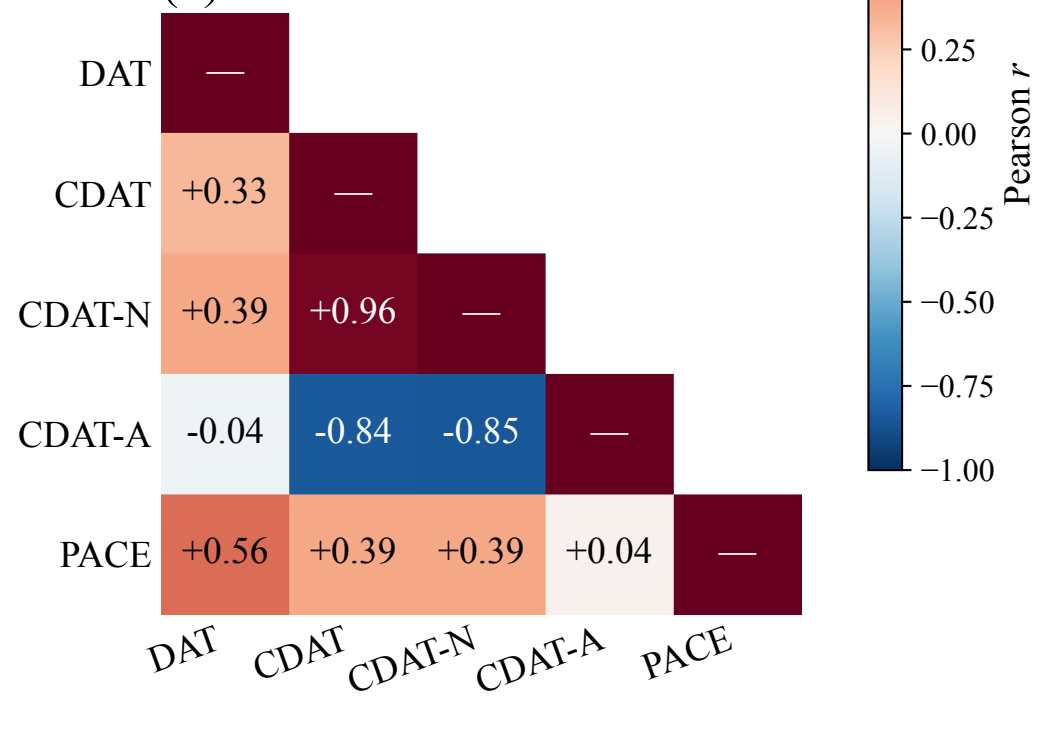
(b) Inter-test correlations
