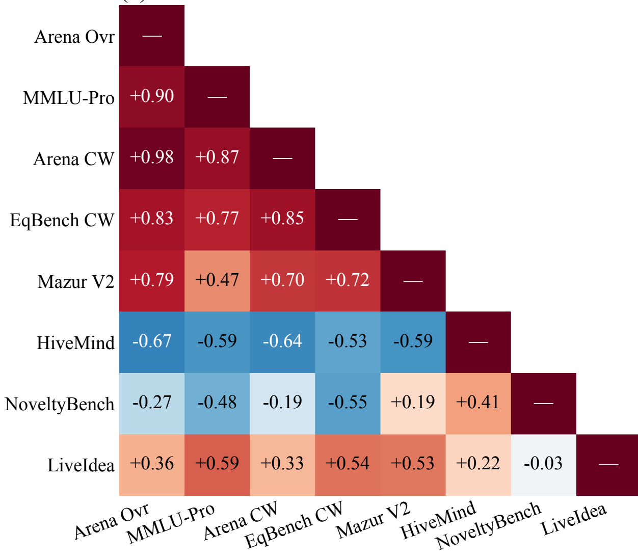
(a) Inter-benchmark correlations
