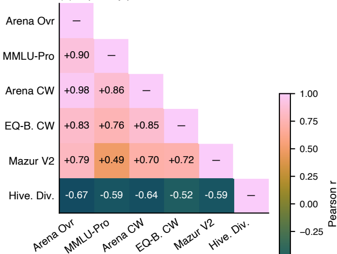
(a) capability proxies + outcome benchmarks
