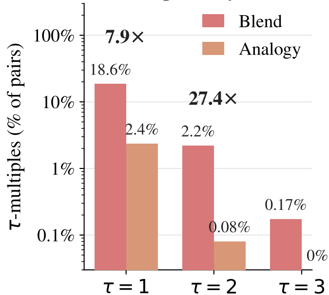
(b) % of pairs, by task
