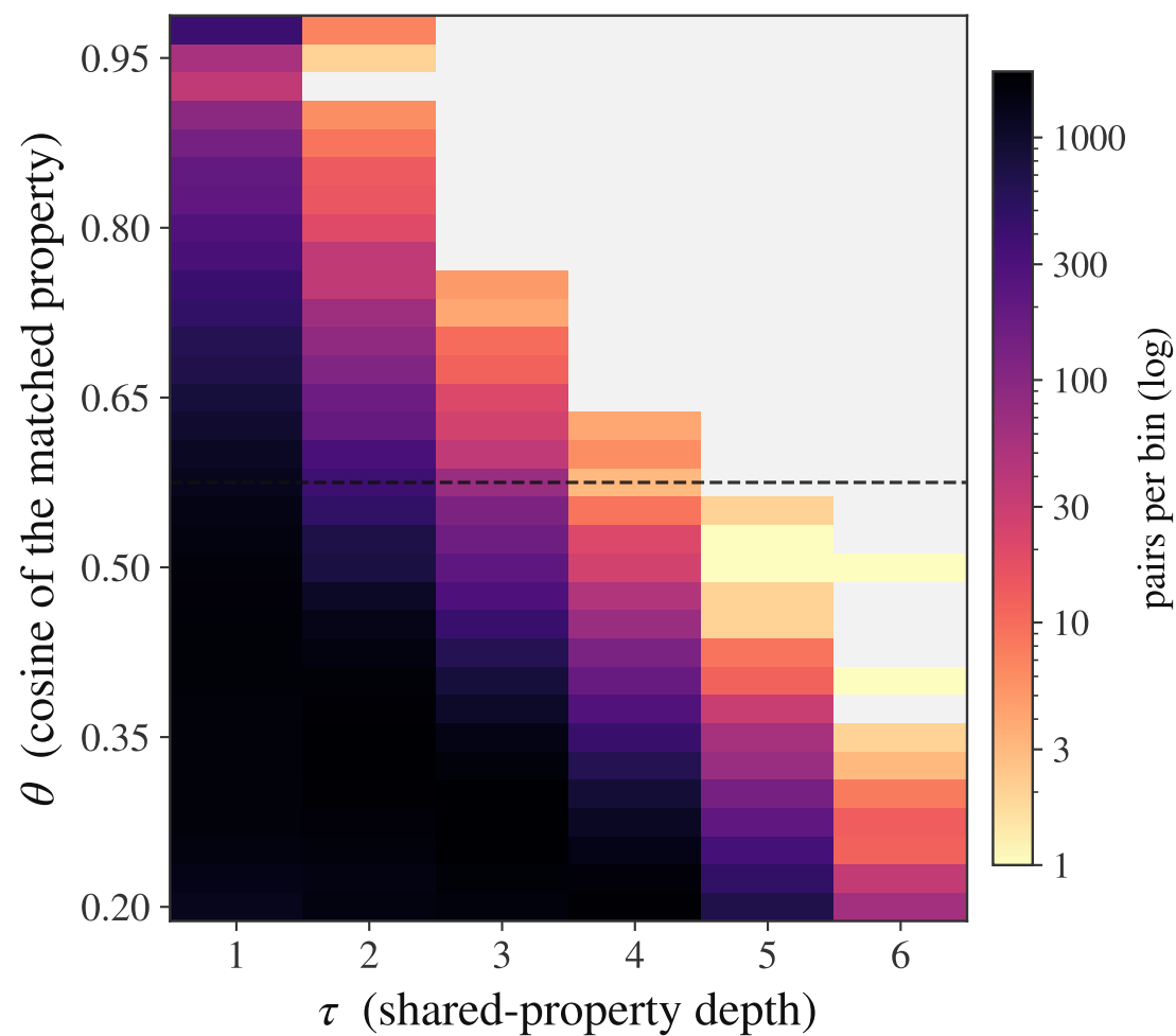
(a) Joint density of shared properties
